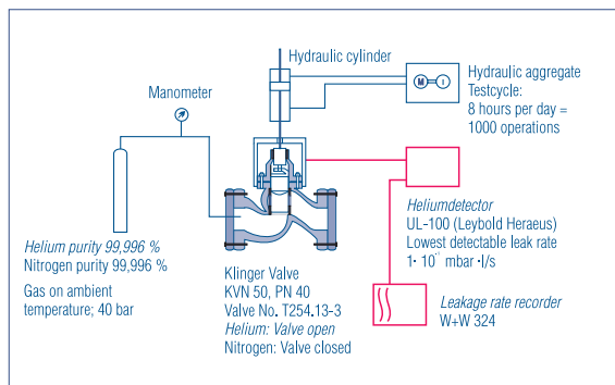
KVN KX1-GT 50.000 cycle test
